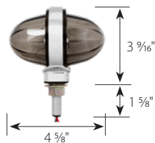
75199 Side view
