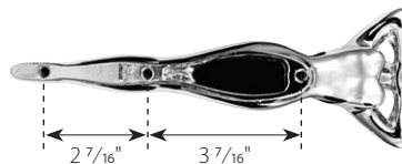
3 Hole bolt pattern
